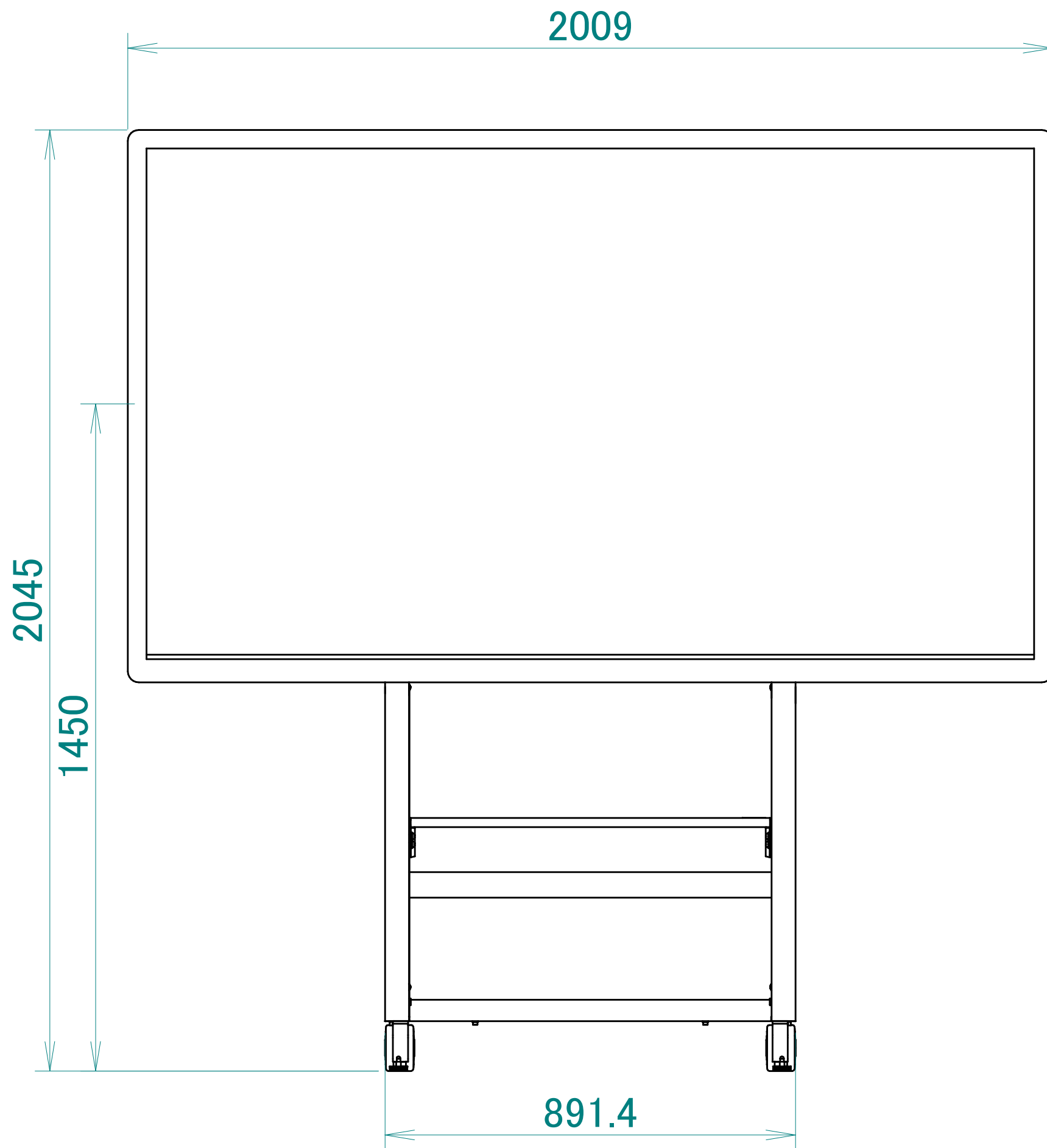
D8600 + Stand Display Center Height: 1450±100mm (1350,1450,1550)
